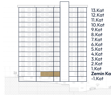
Anahtar Kesit
