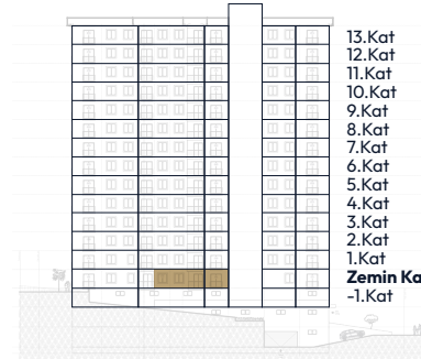
Anahtar Kesit
